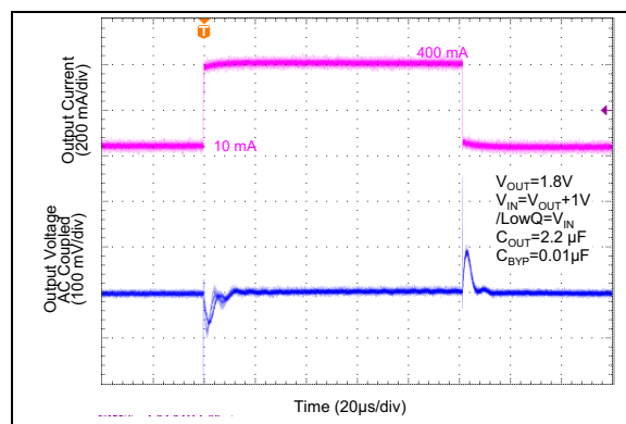
FIGURE 2-23: DC/DC Load Transient PWM Mode.
