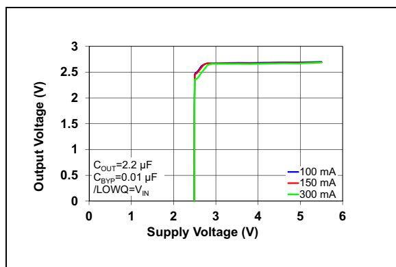
FIGURE 2-20: Dropout Characteristics.
