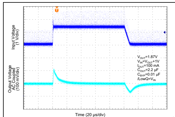
FIGURE 2-24: DC/DC Line Transient PWM Mode.
