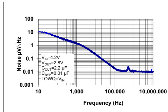
FIGURE 2-22: LDO2 Output Noise Spectral Density.
